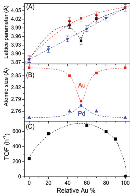
Fig. 4 (A) Atomic PDF-derived “lattice parameters” of the treated under an O 2 atmosphere alone (red circles) and fully activated (black squares) Au 100-x Pd x alloy NPs ( x = 30, 46 and 58 ). Lattice parameters of bulk Au-Pd alloys obtained by traditional powder XRD 49,50 are also shown (down triangles in blue). Note: the “lattice parameters” of Au-Pd NPs evolve rather irregularly with the NP composition. On the other hand, the lattice parameters of bulk Au-Pd alloys evolve linearly with the alloy's composition obeying the so-called Vegard's law. 71 (B) Size of Au (red squares) and Pd (up triangles in blue) atoms that should be used by the SC method in modeling the atomic-level structure of fully activated Au 100-x Pd x alloy NPs ( x = 30, 46 and 58 ) studied here. The size is adjusted against atomic PDFs obtained by total scattering experiments (see the text). (C) Evolution of the catalytic activity of Au-Pd alloy NPs, given in terms of turnover frequency (TOF), for the 2-octen-1-ol oxidation reaction with the NP composition. 7 Broken lines in (A), (B) and (C) are least-squares fits to the respective data points.
