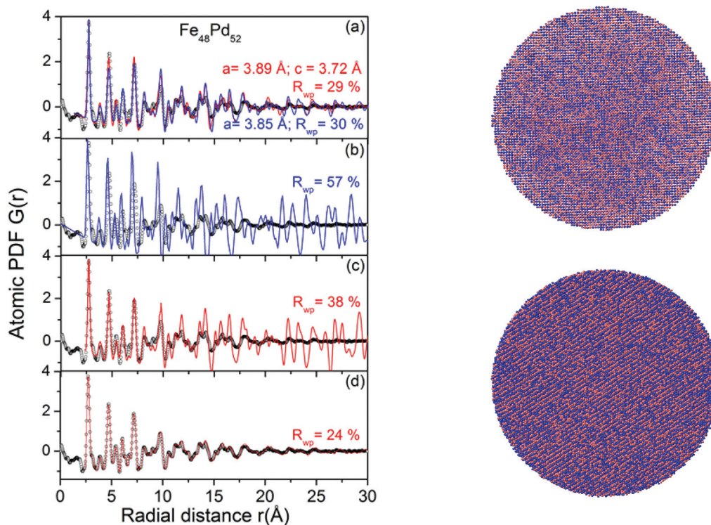
Fig. 9 (Left) Experimental (black symbols) and computed (blue and red lines) PDFs for Fe 48 Pd 52 alloy NPs. The computed PDFs in (a) are based on the fcc- (red line) and tetragonal- (blue line) type crystal structures exhibited by chemically disordered and ordered bulk Fe 100–x Pd x alloys ( x ~ 50), respectively. Values of the NP “fcc- and tetragonal-lattice parameters”, derived by adjusting the structure models against the experimental PDF data, are also given. The computed PDF in (b) is derived from a MD model based on the SC method currently in use (see Table 3). The computed PDF in (c) is derived from a MD model based on the SC method “tuned up” as described in the text. The computed PDF in (d) is derived from a hybrid RMC refined version of the “tuned-up” MD model. Goodness-of-fit indicators, R wp , explained in the ESI,† are shown by each data set in color pertaining to the respective model. (Right top) Structural model for Fe 48 Pd 52 alloy NPs optimized in terms of energy by MD based on the SC method “tuned up” as described in the text. (Right bottom) A hybrid RMC refined version of the MD model. The models comprise 76 495 Fe (brown) and 82 870 Pd (blue) (in total 159 365) atoms.
