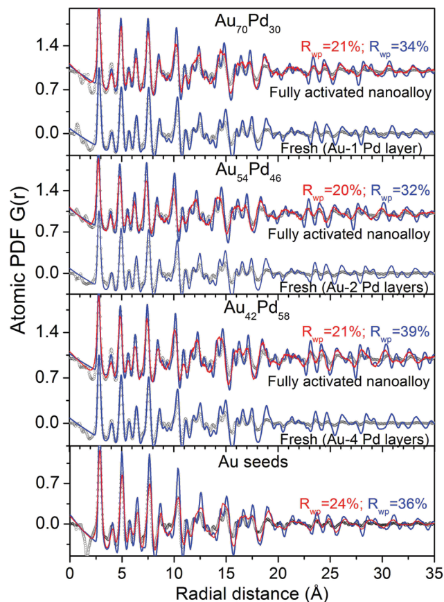
Fig. 7 Experimental (black symbols) and MD (blue lines) model-derived atomic PDFs for Au seeds, fresh (Au core–Pd layer) and fully activated (alloy-type) \text{Au}_{100-x}\text{Pd}_x NPs ( x = 30, 46 and 58 ). The respective MD models are shown in Fig. 6 (left). Atomic PDFs derived from the hybrid RMC further refined versions (see Fig. 6, right) of MD models are also shown (red lines). The model's goodness-of-fit indicators, R_{\text{wp}} , explained in the ESI,† are shown by each data set in color pertaining to the respective model-derived PDF. The MD models produce atomic PDFs that match the respective experimental data quite well, except for the region of higher- r values. The experimental data are reproduced best by the hybrid RMC further refined models, as a visual inspection and the values of respective R_{\text{wp}} indicators are shown.
