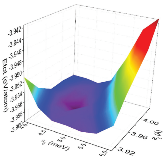
Fig. 5 Energy, E_{\text{tot}} , of the set of “trial” models for fully activated Au 42 Pd 58 alloy NPs generated by a series of MD runs performed as described in the text. In particular, in the simulations the value of the SC parameter \epsilon_{ij} , i.e. the strength of the interaction between Au and Pd atoms, and the value of the SC parameter a_{ij} , i.e. the bonding distance between Au and Pd atoms, have been systematically varied within the range of values of the currently used SC parameters \epsilon_{ii} and a_{ii} for Au and Pd atoms (listed in Table 1), respectively. An MD model based on SC parameters \epsilon_{ij} and a_{ij} derived as a harmonic average of the currently used SC parameters \epsilon_{ii} and a_{ii} for Au and Pd atoms, respectively, appears of lowest energy (−3.96 eV per atom) as compared to all other MD models tried. For reference, the binding energy of bulk Au is −3.81 eV per atom and that of bulk Pd is −3.89 eV per atom.
