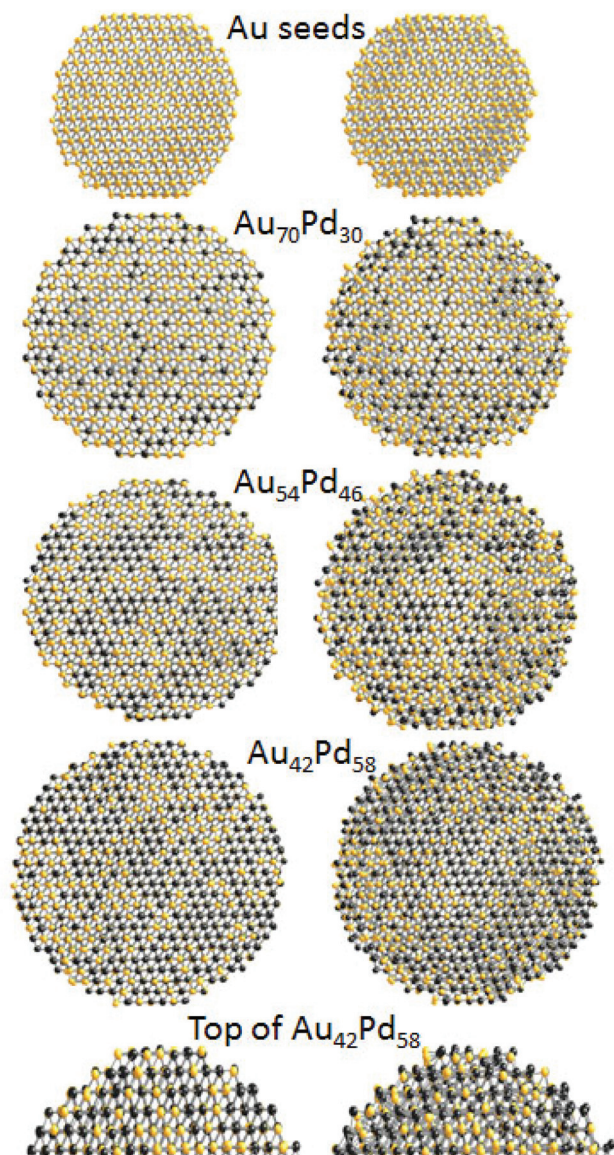
Fig. 6 (Left) 3D structural models for Au seeds and fully activated \text{Au}_{100-x}\text{Pd}_x alloy NPs ( x = 30, 46, 58 ) built by MD simulations based on the SC method/parameters "tuned up" against experimental PDF data as described in the text. The models feature random alloy NPs wherein Au and Pd atoms are fcc-like arranged locally. (Right) Hybrid RMC refined versions of the MD models shown on the left. Corresponding segments of the surface of the MD built and hybrid RMC further refined model for \text{Au}_{42}\text{Pd}_{58} NPs are also shown (at the very bottom) to make clearer the virtual absence and very presence of near-surface structural disorder in the former and latter models, respectively. Au atoms are in yellow and Pd atoms are in black.
