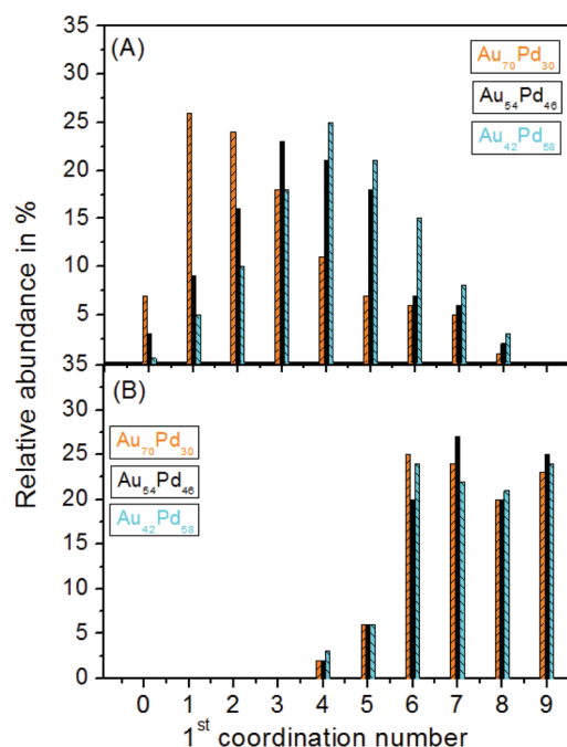
Fig. 10 Distribution of the first (A) Pd-Pd and (B) total coordination numbers for atoms at the surface of fully activated \text{Au}_{100-x}\text{Pd}_x ( x = 30, 46, 58 ) NPs as extracted from their 3D models shown in Fig. 6, right.
