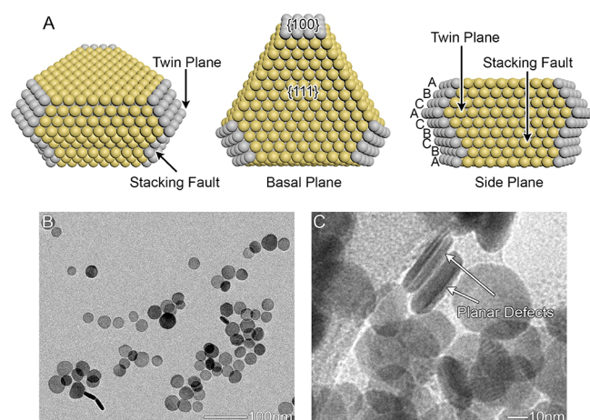
Figure 5. (A) Simplified schematic of the structure of silver nanodisks (nanodisks) in which the basal planes are {111} facets and the side planes contain a mixture of {100} facets, {111} facets, and planar defects. (B) TEM image of silver nanodisks and (C) HRTEM image of the planar defects in silver nanodisks.
